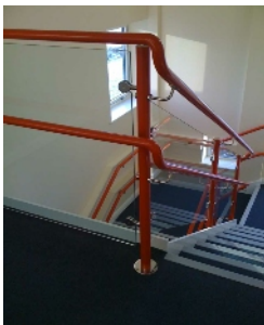
Glazed Stargard with “double” handrail and glass infill panels
